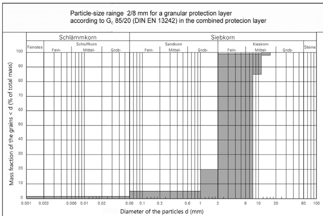
Figure 1: Preferred particle-size range for a granular protection layer fulfilling geometric filter criteria in the combined protection layer.
