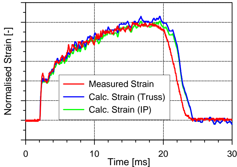
Figure 1. Comparison of measured and calculated strains (cask body inside, opposite to the puncture bar impact, GNS-CASTOR HAW28M/TB2 drop test horizontally onto a steel bar-75 mm diameter [2])
