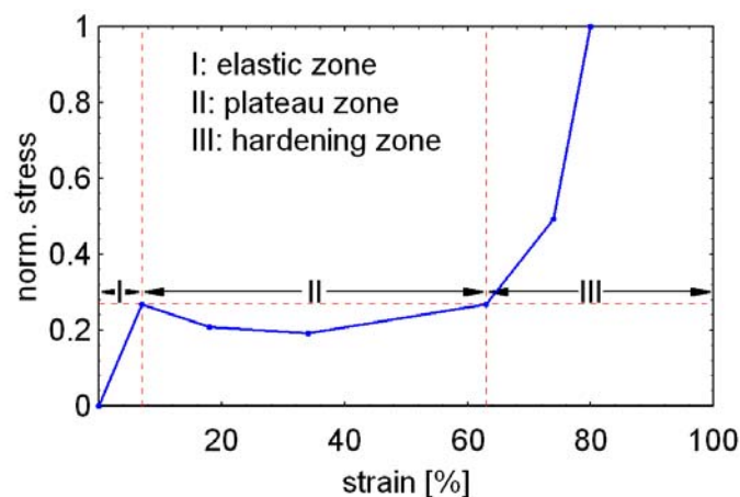
Figure 2. Yield curve of wood
