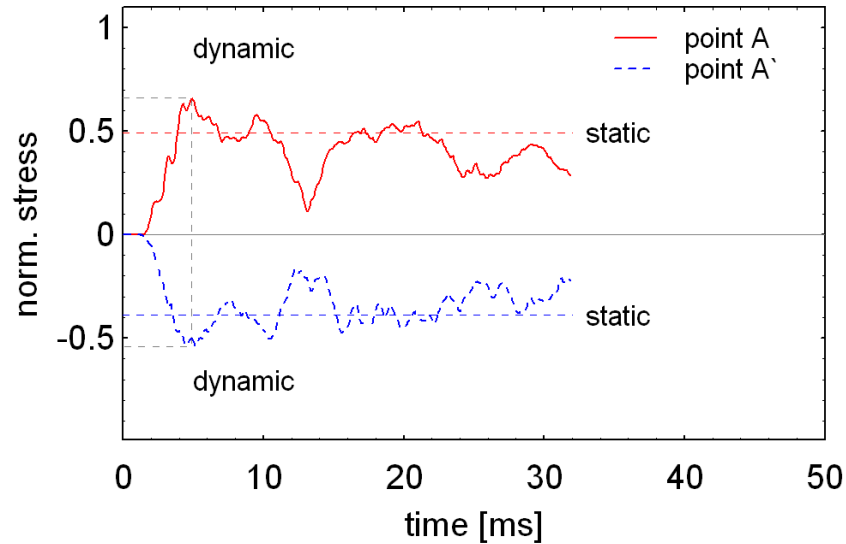
Figure 4. Normalised stresses at the middle of reference cask body (at points A, A'-Fig. 3b; 9m horizontal drop test)
