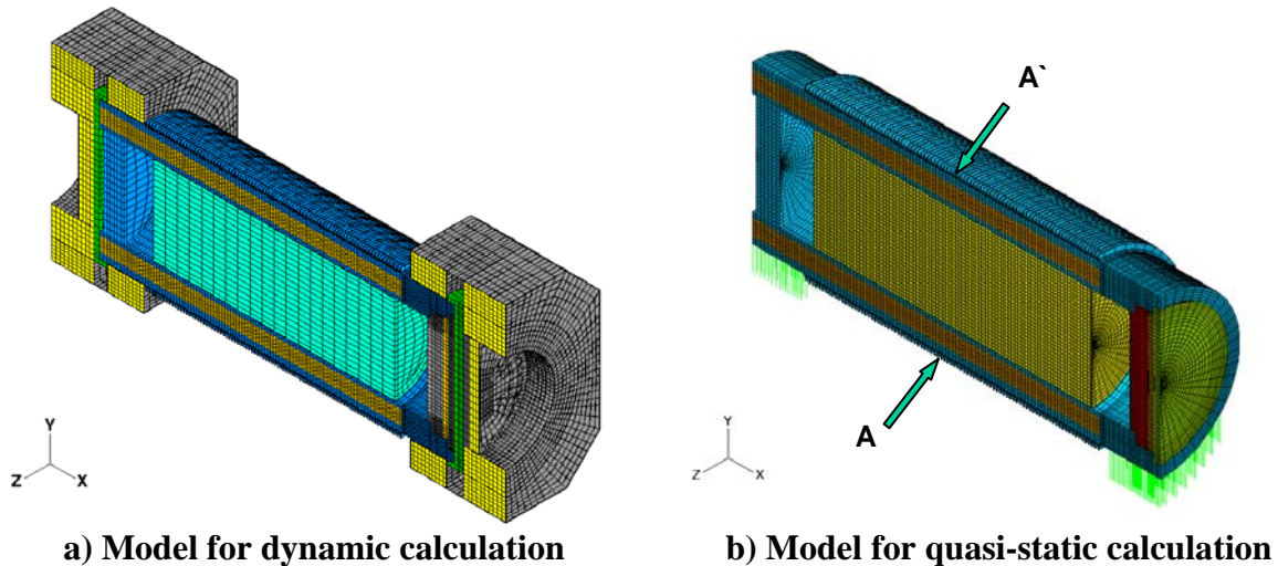
Figure 3. Reference package model for dynamic and quasi-static calculation
